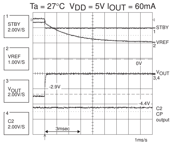
(b) 50Ω - Falling waveform
