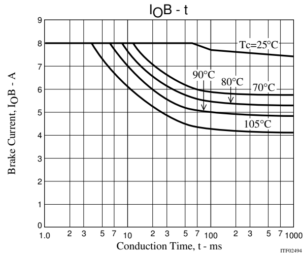
STK681-320 Allowable Brake Current Range
