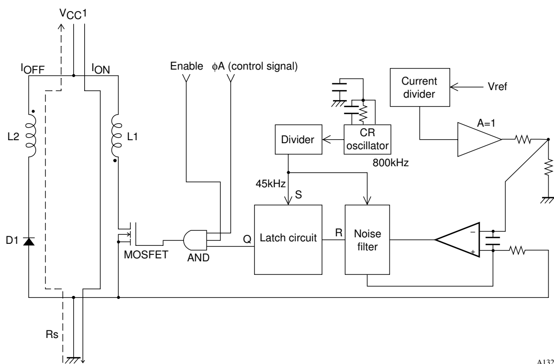
Driver Block Basic Circuit Structure
