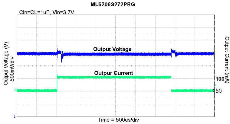
Load Current 50mA to 100mA
