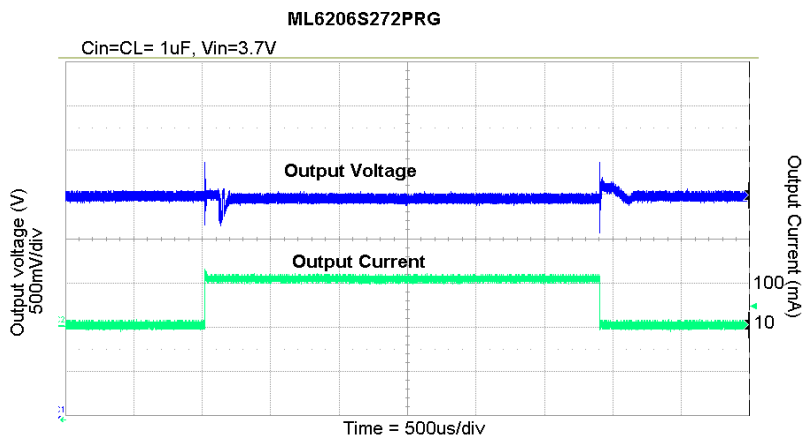
Load Current 10mA to 100mA
