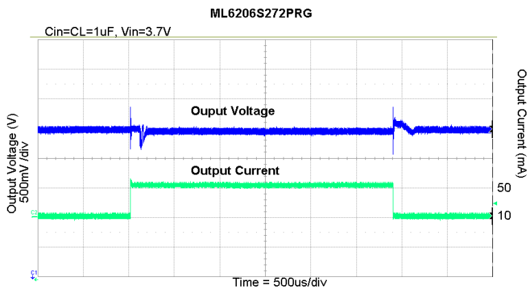
Load Current 10mA to 50mA
