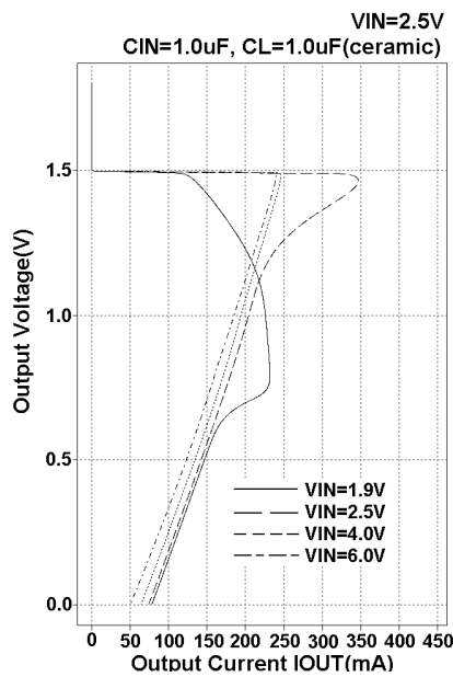
ML6206S153
