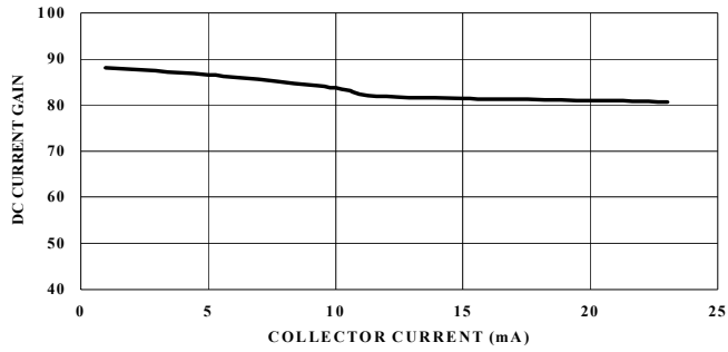
DC CURRENT GAIN ( h_{FE} ) vs COLLECTOR CURRENT at VCE = 3 V
