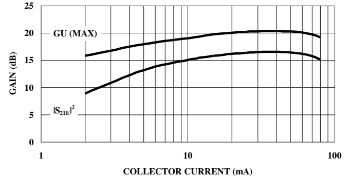
MP4T85600 NOMINAL GAIN vs COLLECTOR CURRENT at F = 1GHz and V CE = 8 VOLTS
