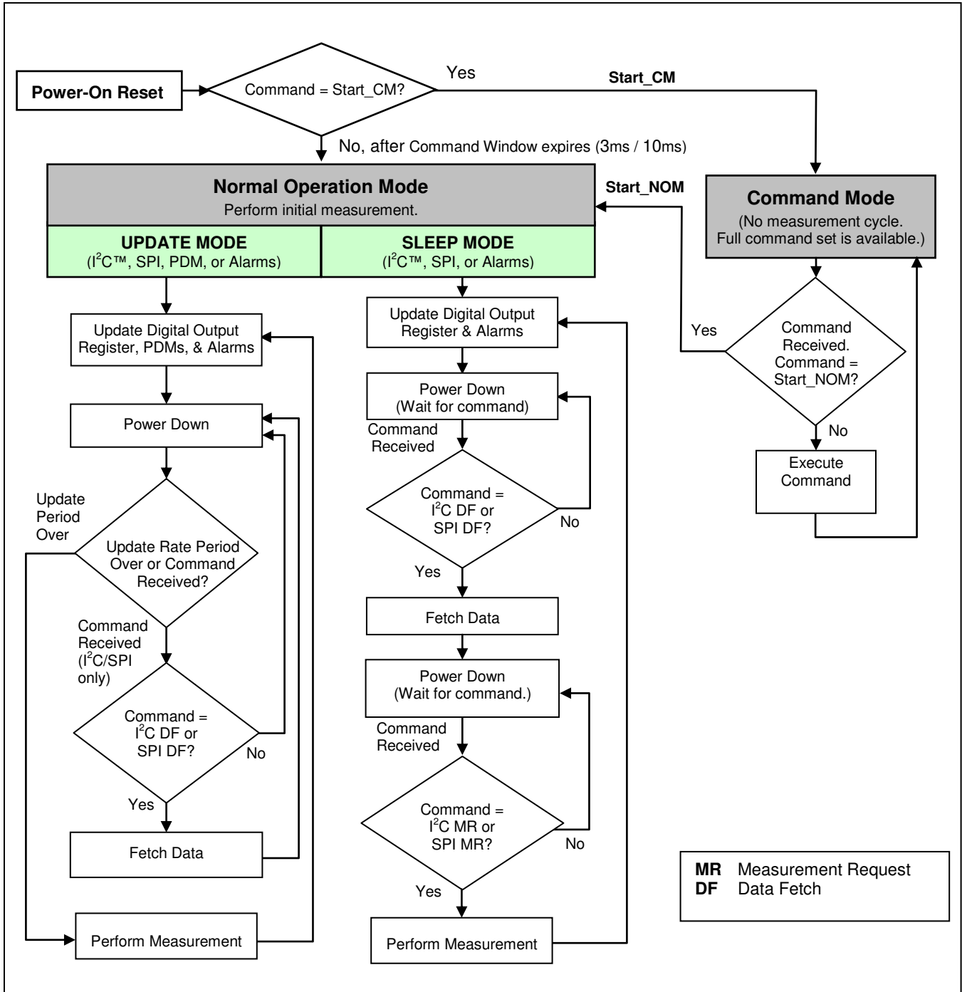
Figure 3.1 General Operation
