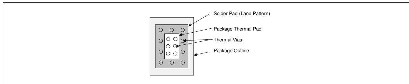
Figure 6.2 Package and PCB Land Configuration for Multi-Layer PCB
