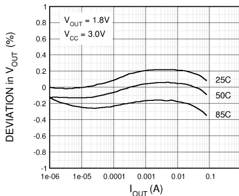
Figure 2.8 Load Regulation Performance
