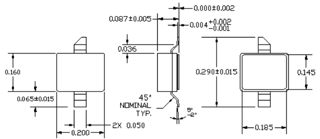
PACKAGE DIMENSIONS IN INCHES
