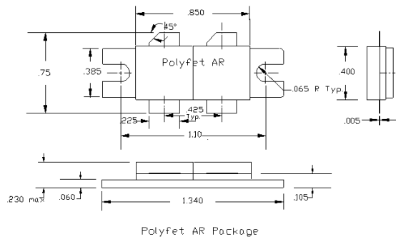
PACKAGE DIMENSIONS IN INCHES
