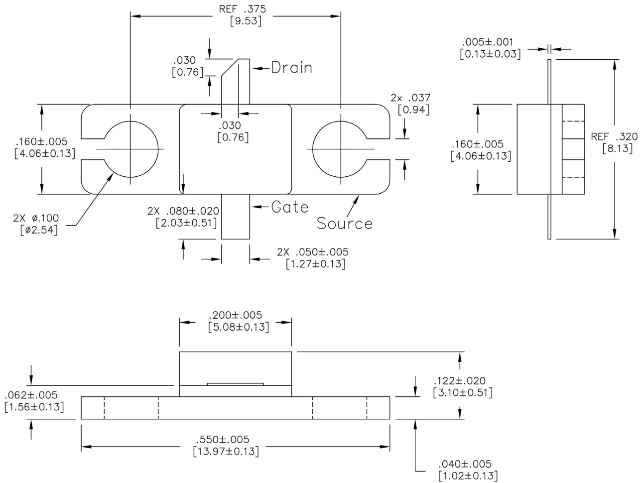
Figure 18 - AC200B-F2 Package Dimensions and Pinout (all dimensions are in inches)
