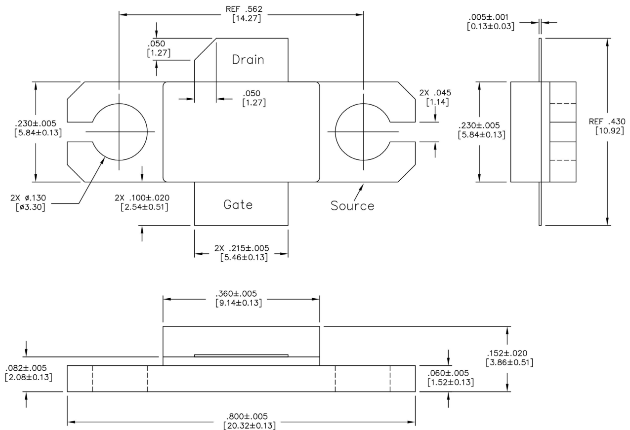
Figure 8 - AC360B-F2 Package Dimensions and Pinout (all dimensions are in inches)
