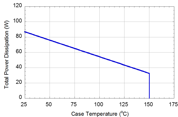
Figure 8: Power De-rating Curve ( T_J = 225^\circ C , T_C > 25^\circ C )
