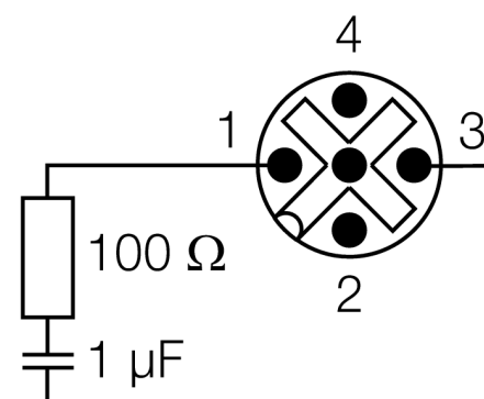
Wiring diagram
