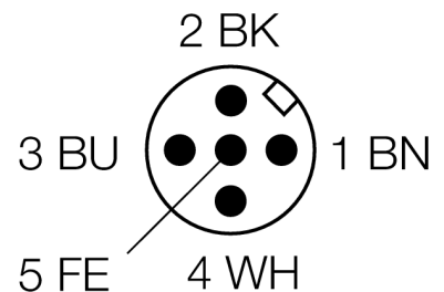
Pin assignment right
