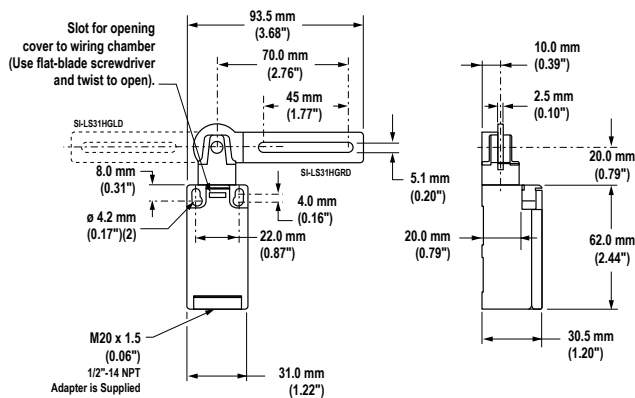
Models SI-LS31HGRD/HGRE and HGLD/HGLE
