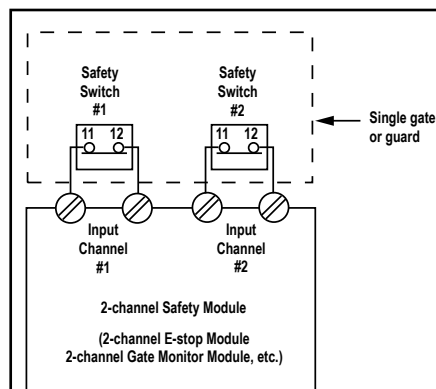
Figure 2. Door opens in one direction
