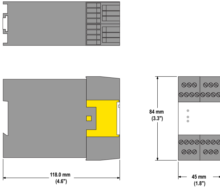
Figure 4. Dimensions, in mm (inches)
