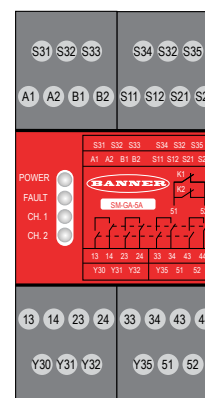
Figure 1. Indicator and Terminal Locations
