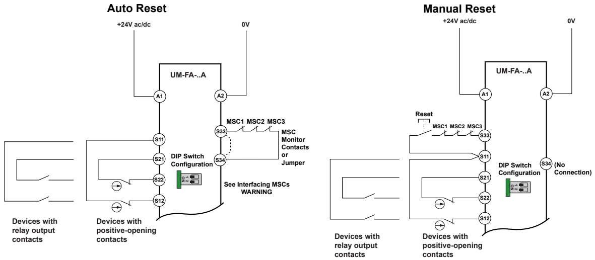
Dual-Channel Hookup Configuration for Devices with Hard Contacts
