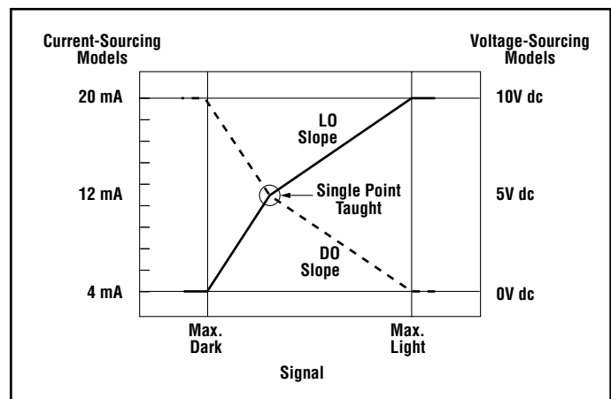
Figure 3. Analog output as a function of target position – single-point TEACH
