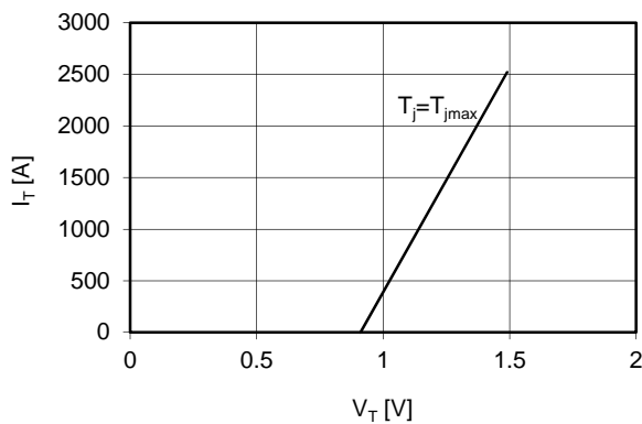
On-state voltage drop
