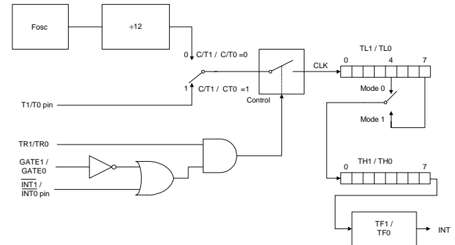
FIGURE 6: TIMER/COUNTER 1 MODE 0: 13-BIT COUNTER
