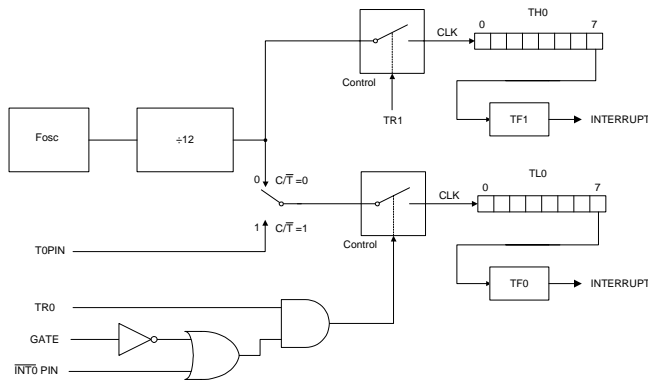
FIGURE 8: TIMER/COUNTER 0 MODE 3
