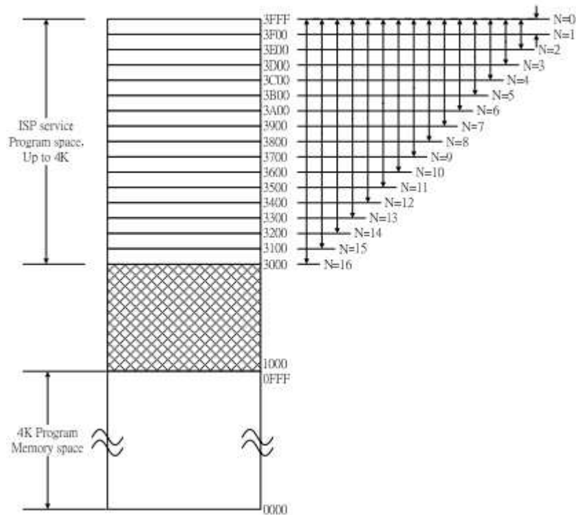
Fig.3.1: Flash Memory Structure
