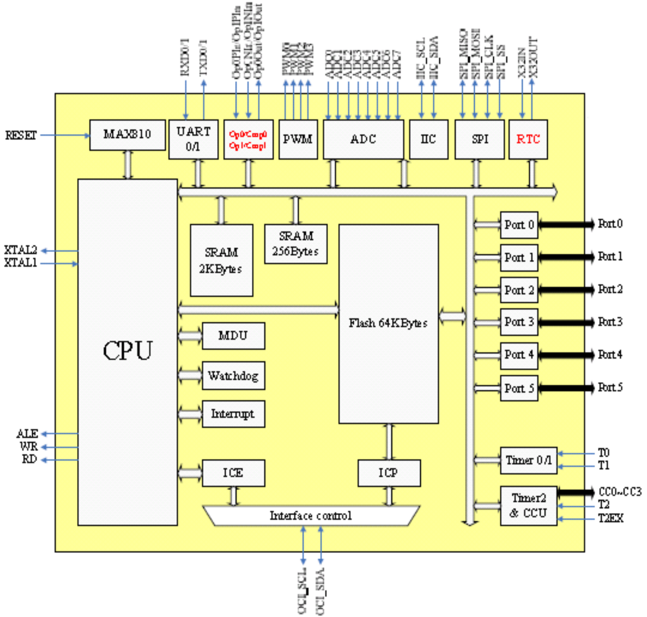
Fig. 1-1. Device Block Diagram
