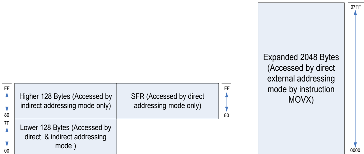
.Fig. 3-3: RAM architecture
