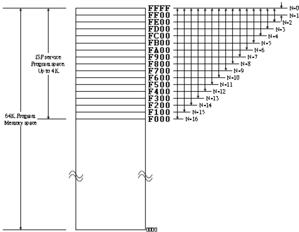
Fig.3.1: Flash Memory Structure
