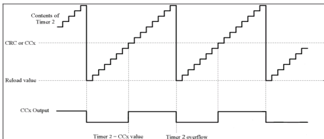
Fig. 8-1: Compare mode 0 function
