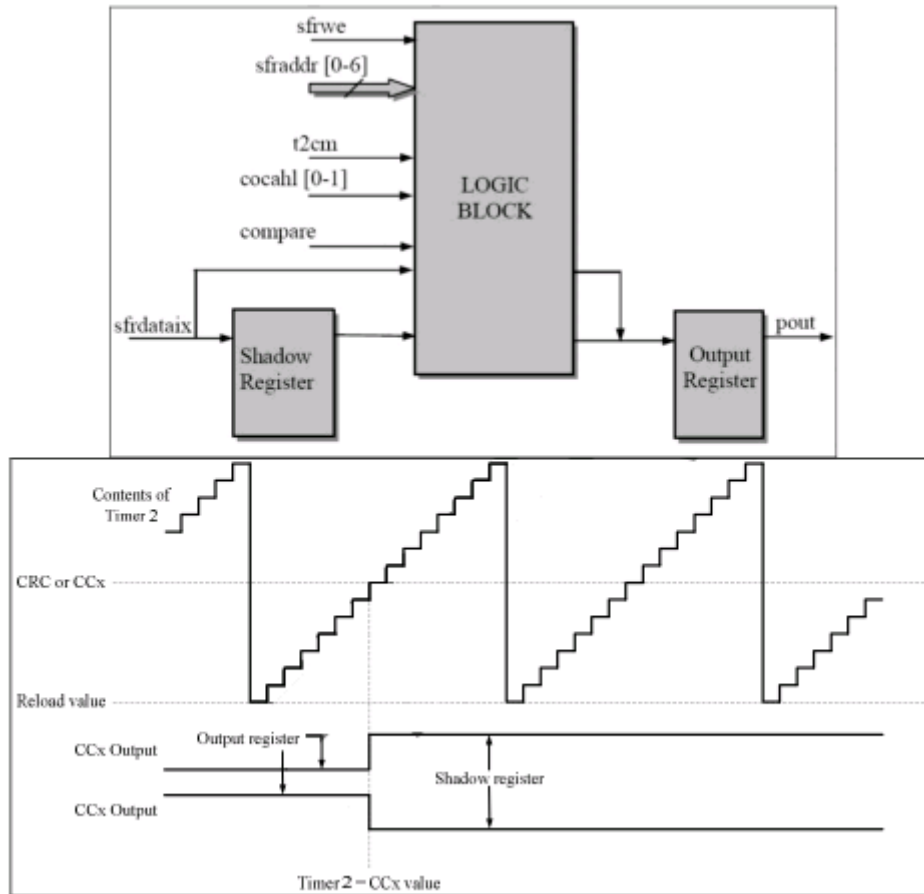
Fig. 8-2: Compare mode 1 function
