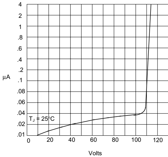
Instantaneous Reverse Current - Micro Amps versus Percent Of Rated Peak Reverse Voltage - Volts
