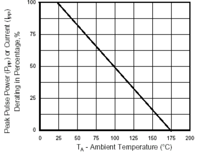
Fig.2-Power Derating Curve
