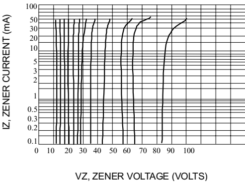
Fig. 8-VZ = 12 THRU 82 VOLTS
