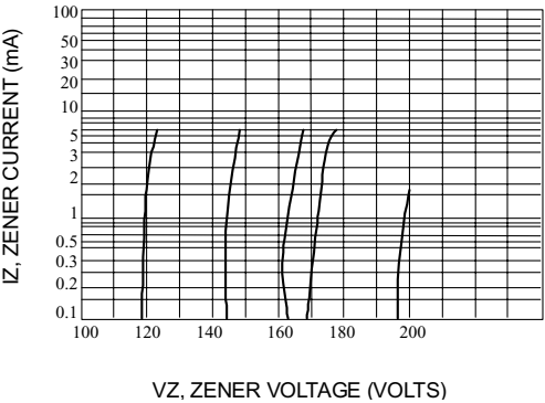
Fig. 9-VZ = 100 THRU 200 VOLTS
