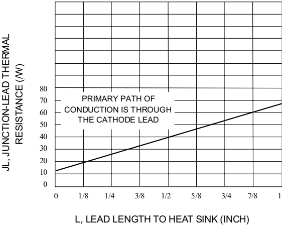
Fig. 10-TYPICAL THERMAL RESISTANCE
