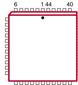
44-Lead Quad Plastic Chip Carrier (PJ)
