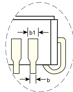
View B
