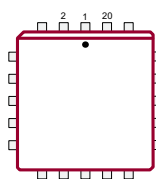
20-Lead PLCC (PJ) (top view)
