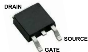
3-Lead TO-252 (D-PAK) (K4)
