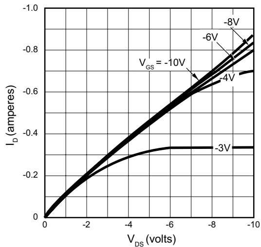
Saturation Characteristics
