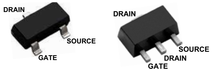
TO-236AB (SOT-23) (K1)
