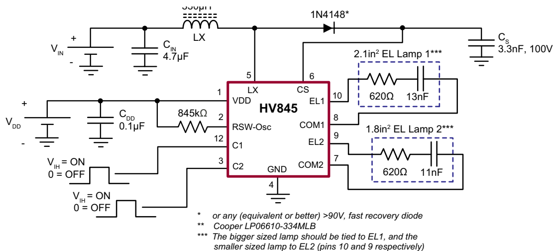
Fig. 1 - Test Circuit
