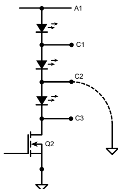
Fig.1 : Short Cathode Fault
