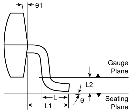
View B
