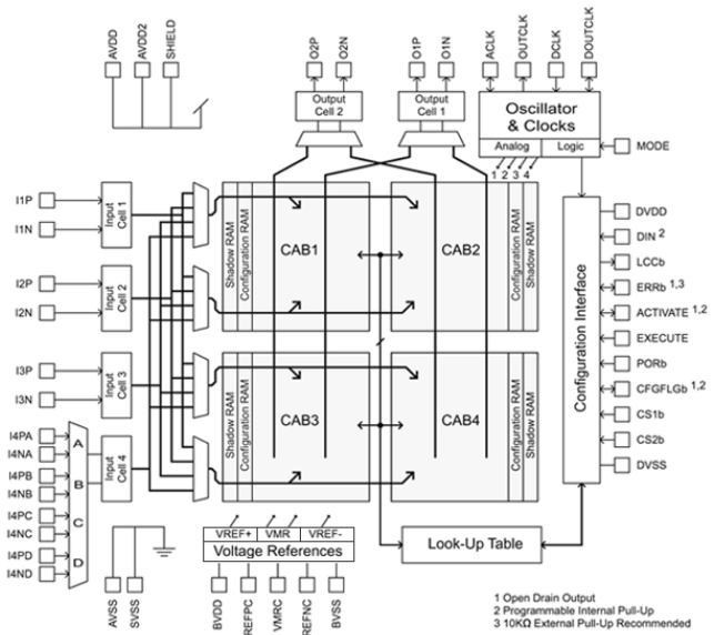
Figure 1: Architectural overview of the AN120E04 device
