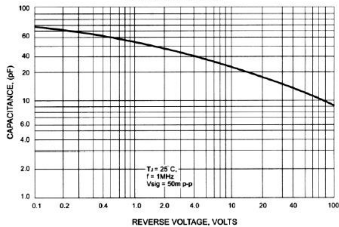
FIG. 5 - TYPICAL JUNCTION CAPACITANCE PER BRIDGE ELEMENT
