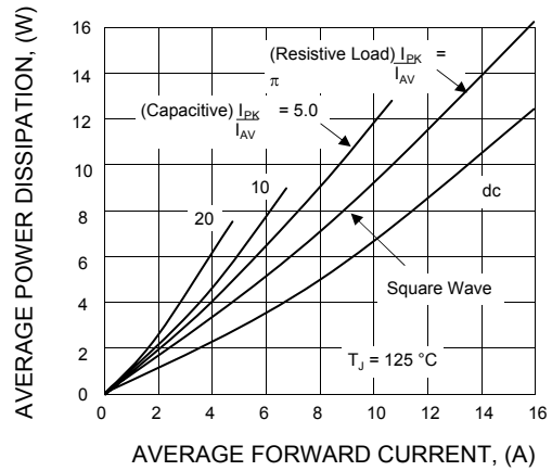
FIG.2 - POWER DISSIPATION
