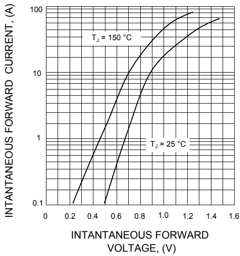
FIG.3 - TYPICAL FORWARD VOLTAGE
