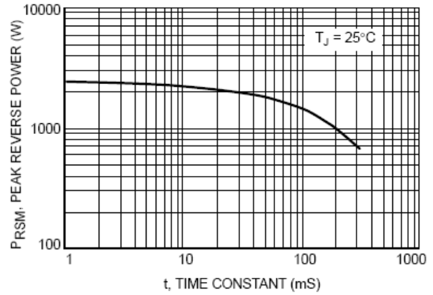
FIG.10 - REVERSE POWER DERATING
