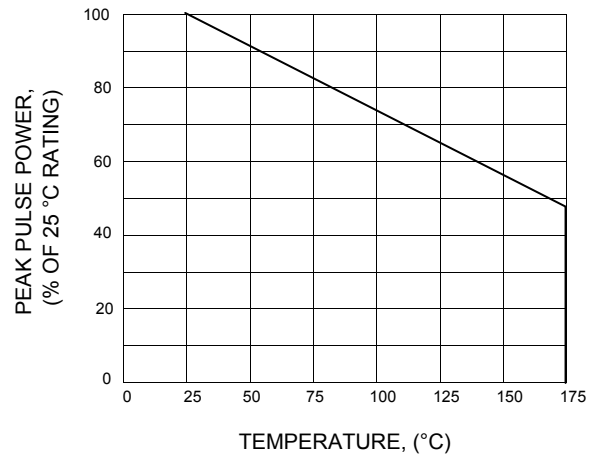
FIG.2 - DREATING CURVE
