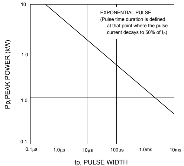
FIG.4 - PEAK PULSE POWER VS. PULSE DURATION
