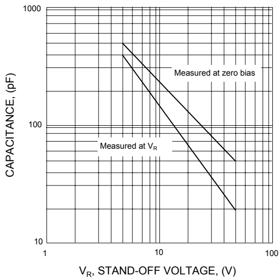
FIG.3 - TYPICAL CAPACITANCE VS. STAND-OFF VOLTAGE
