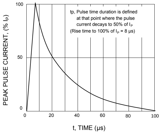
FIG.1 - CURRENT IMPULSE WAVEFORM
