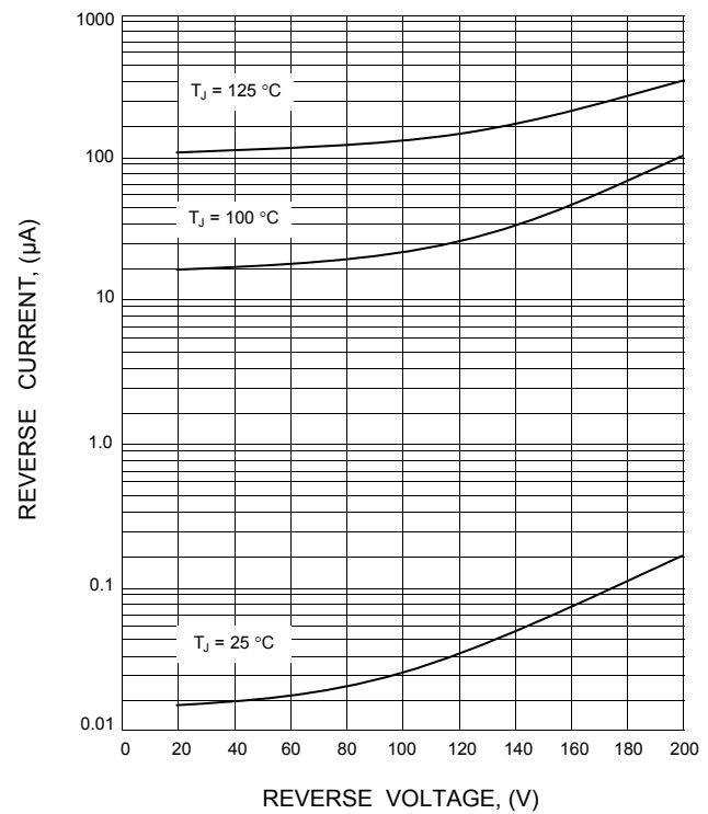
FIG.2 - TYPICAL REVERSE CHARACTERISTICS (PER LEG)
