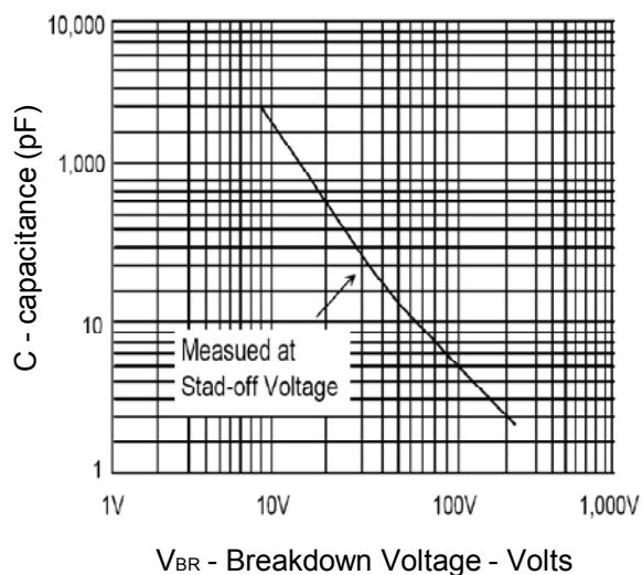
FIG.3 - TYPICAL CAPAITANCE VS. BREAKDOWN VOLTAGE
