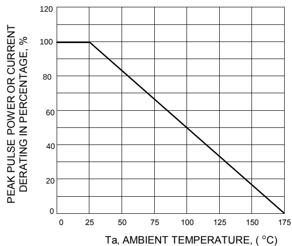
FIG.4 - PULSE DERATING CURVE
