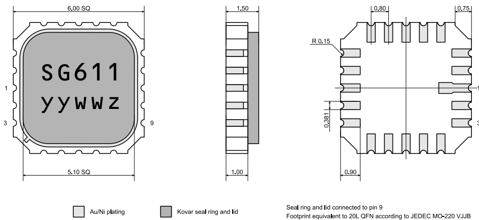
20L CQFN package drawing
