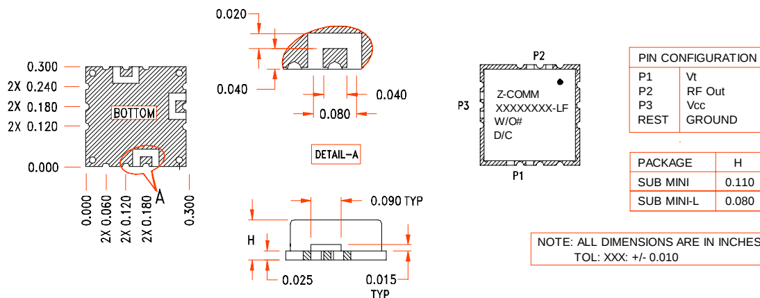
Physical Dimensions
