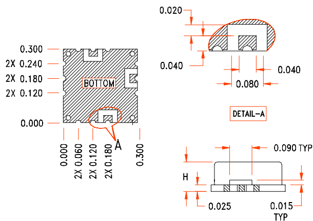
Physical Dimensions
