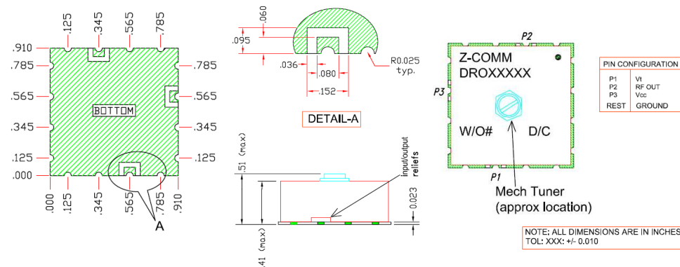
Physical Dimensions
