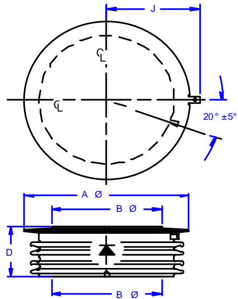
MECHANICAL OUTLINE
