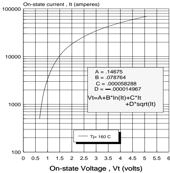
MAXIMUM FORWARD CHARACTERISTIC
