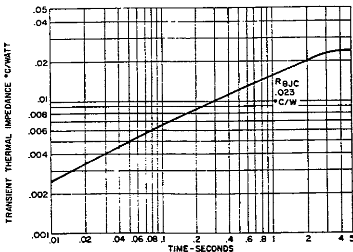
10. TRANSIENT THERMAL RESISTANCE - JUNCTION-TO-CASE
