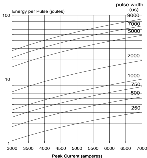
ENERGY LOSS PULSE / C770 THYRISTOR Half sine pulses / No reverse loss
