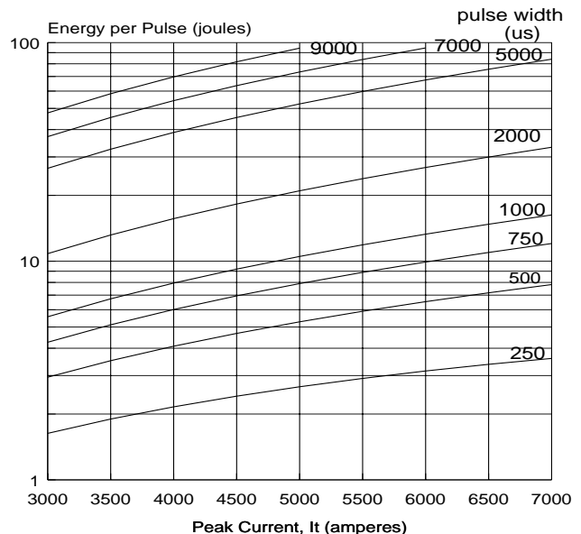
ENERGY PER PULSE Trapezoidal Wave - no reverse voltage di/dt = 100 \text{ A/us}
