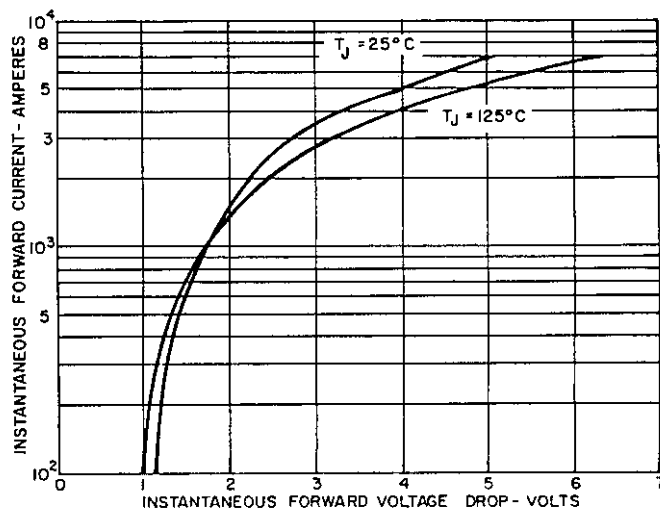
10. FORWARD CONDUCTION CHARACTERISTIC, ON-STATE
